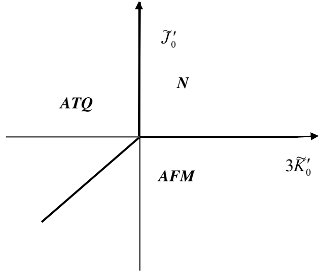
Fig. 2. Phase diagram of two-sublattice non-Heisenberg spin-2 magnetic on the (\tilde{J}', \tilde{K}') -plane.
