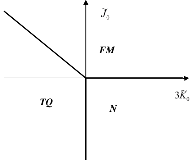
Fig. 1. Phase diagram of non-Heisenberg spin-2 ferromagnetic on the (\tilde{J}_0, \tilde{K}_0) -plane.
